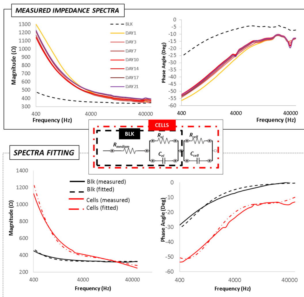
Fig. 4. Impedance-based cell monitoring vs frequency and spectra fitting with equivalent circuit: a) Impedance magnitude and phase spectra vs frequency during the differentiation process. b) Equivalent circuit of blank and seeded sensors used to fit the spectra.
