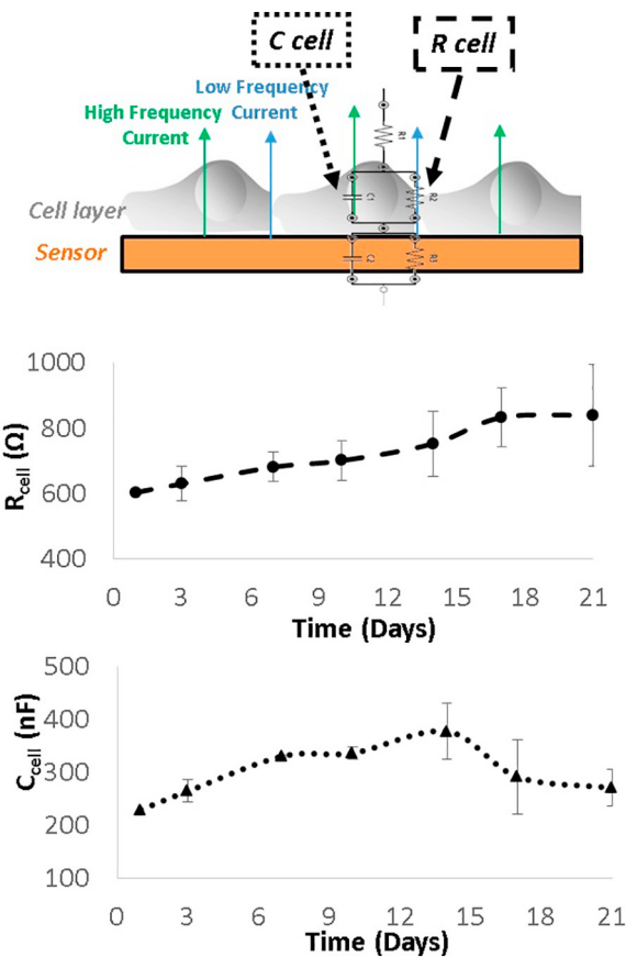
Fig. 5. Evolution of R_{cell} and C_{cell} during differentiation: above, schematic of correspondence between the different parameters in the model with the circuit element; below, specific evolution of the modeling circuit parameters related to cells attached on the sensors.
