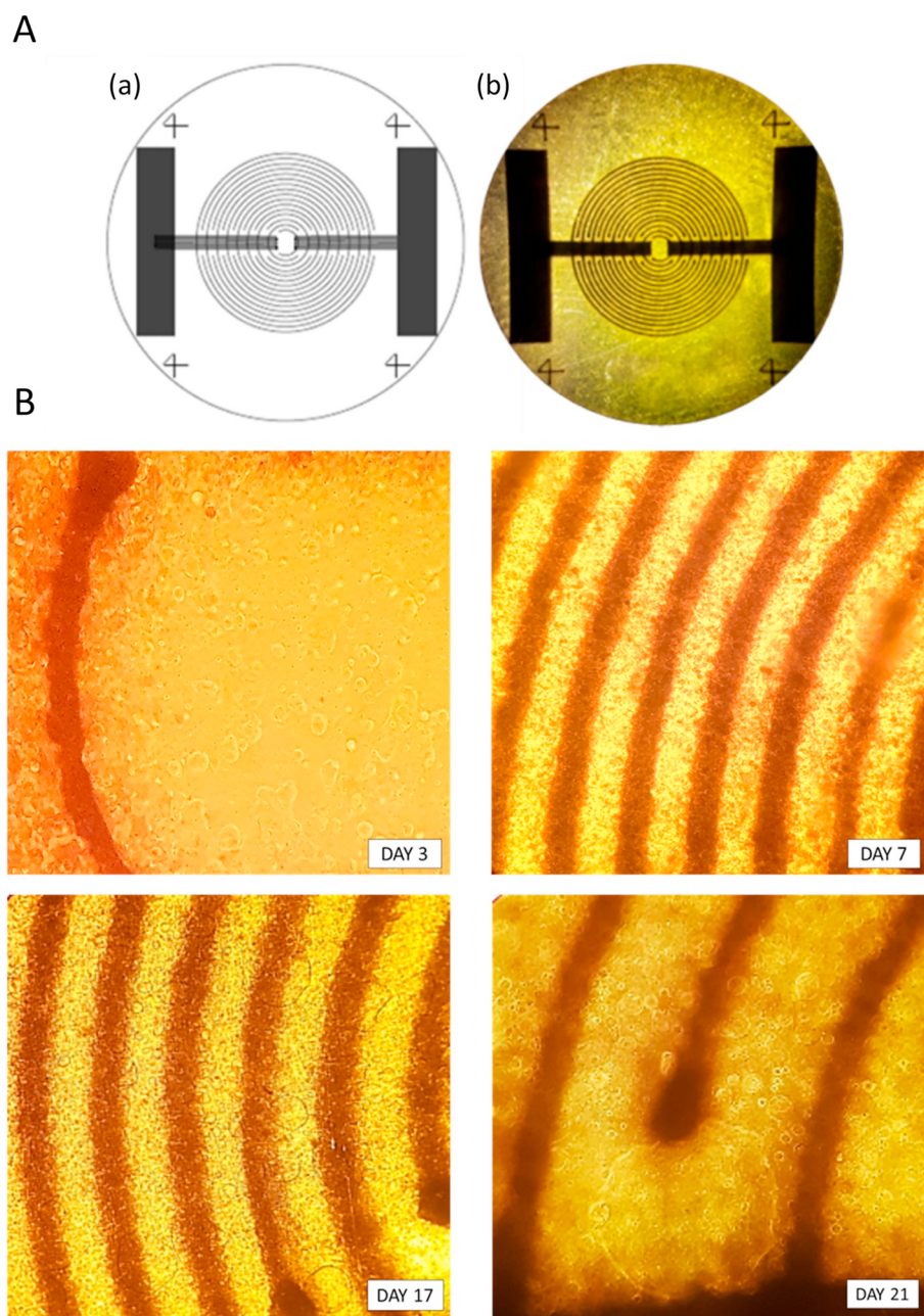
Fig. 2. Caco-2 to enterocyte-like cells differentiation on interdigitated carbon-based electrodes printed on a polyimide substrate. A) Printed Sensor geometry optimized with AutoCAD 2017 (a) and image of the sensor acquired with microscope (magnification 1\times ) (b). B) Representative pictures of Caco-2 cells evaluation at four different time-points (days 3–7–17–21) during 21 days differentiation protocol (magnification 10\times and 20\times for day 21) where sensor geometry is clearly visible. The 21 day picture results out of focus to better visualize the domes.
